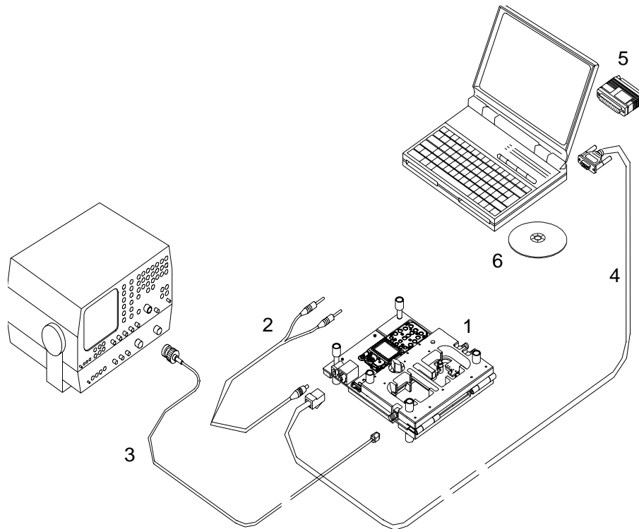
Figure 4: Jig Concept
