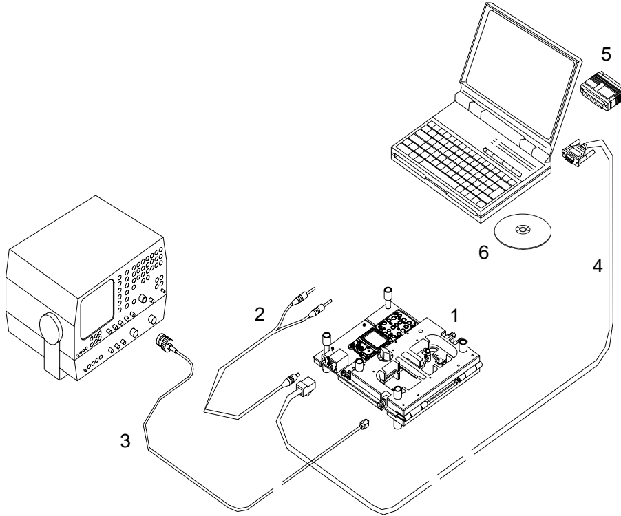
Figure 5: CPL-9 Service Concept
