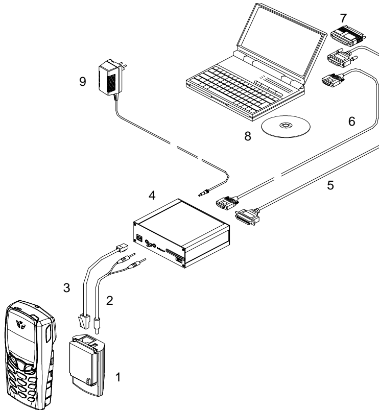
Figure 1: Flash Concept
